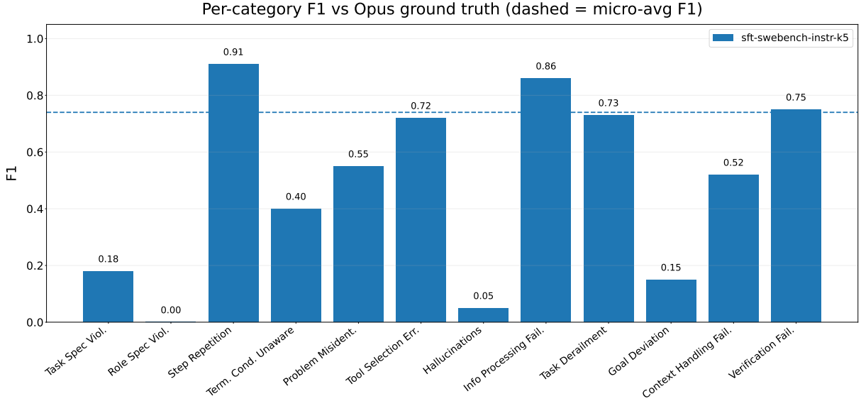
Figure 5: Error categorization results.
