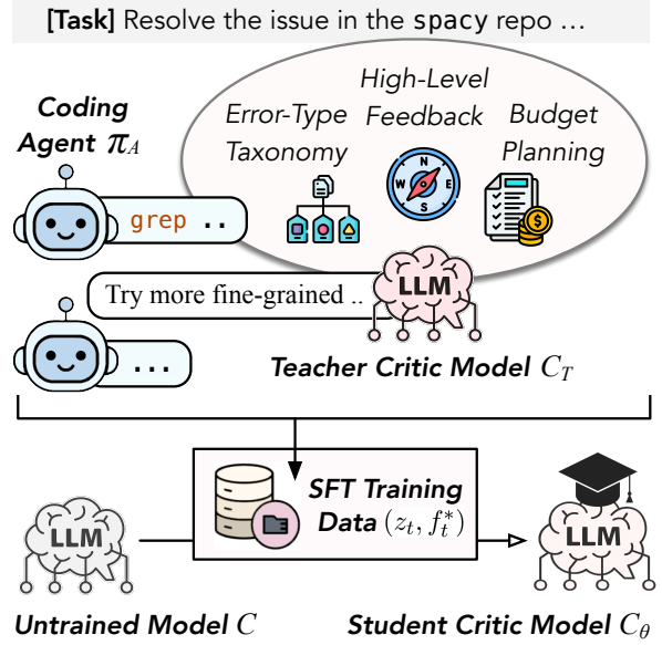
Figure 2: SFT training pipeline for critic models. Based on our analysis (§2.2), the critic contains error detection, budget planning, and only provides high-level feedback instead of concrete actions. We run the frozen coding agent \pi_A on disjoint training tasks and query the teacher critic C_T every k steps. We collect (trajectory prefix, feedback) pairs (z_t, f_t^*) to train a critic C_\theta by supervised fine-tuning (SFT).
