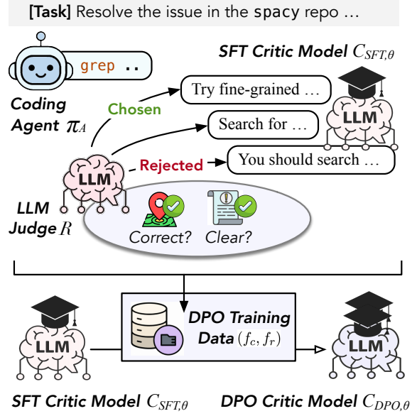
Figure 3: DPO training pipeline for critic models. Given a critic model checkpoint C_{SFT,\theta} , for every k steps produced by the coding agent \pi_A , we use C_{SFT,\theta} to generate N = 10 critiques, and prompt an LLM judge model R to select the best and worse critique, which forms (chosen, rejected) pairs (f_c, f_r) to train C_{SFT,\theta} by direct preference optimization (DPO). We only keep a (f_c, f_r) pair if the chosen critique is both correct and provides clear instruction and the rejected critique misses any of the criteria.
