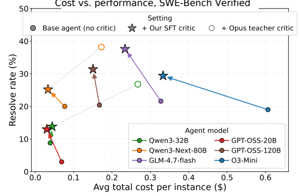
Figure 4: Cost versus performance on SWE-Bench Verified across six coding agents. Each agent shows its base (●) and the 8B SFT critic (★); the two Qwen agents additionally show the Claude-Opus-4.6 teacher critic (○). The cost is for the agent plus the critic model.
