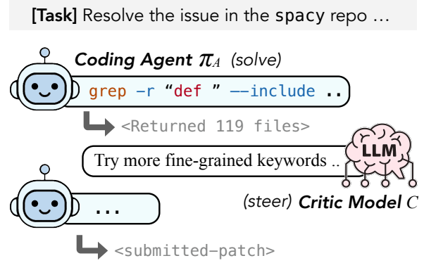
Figure 1: Inference setup. A trained critic model C provides guidance to a frozen coding agent \pi_A for every k steps. The agent is responsible for all concrete actions and the critic model inspects the current trajectory and generates high-level feedback for its next steps.
